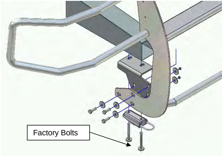
Figure 1.2 – Passenger-Side Mount Bracket
